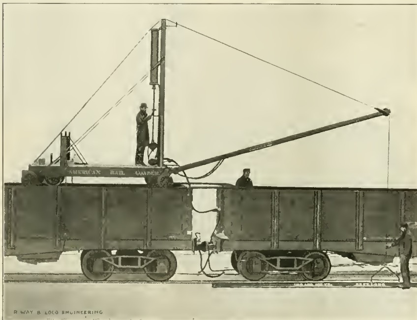
AIR OPERATED RAIL LOADER.
